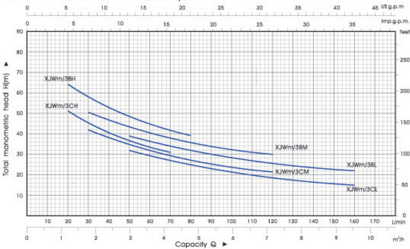
PERFORMANCE CHART AT n=2900 1/min
